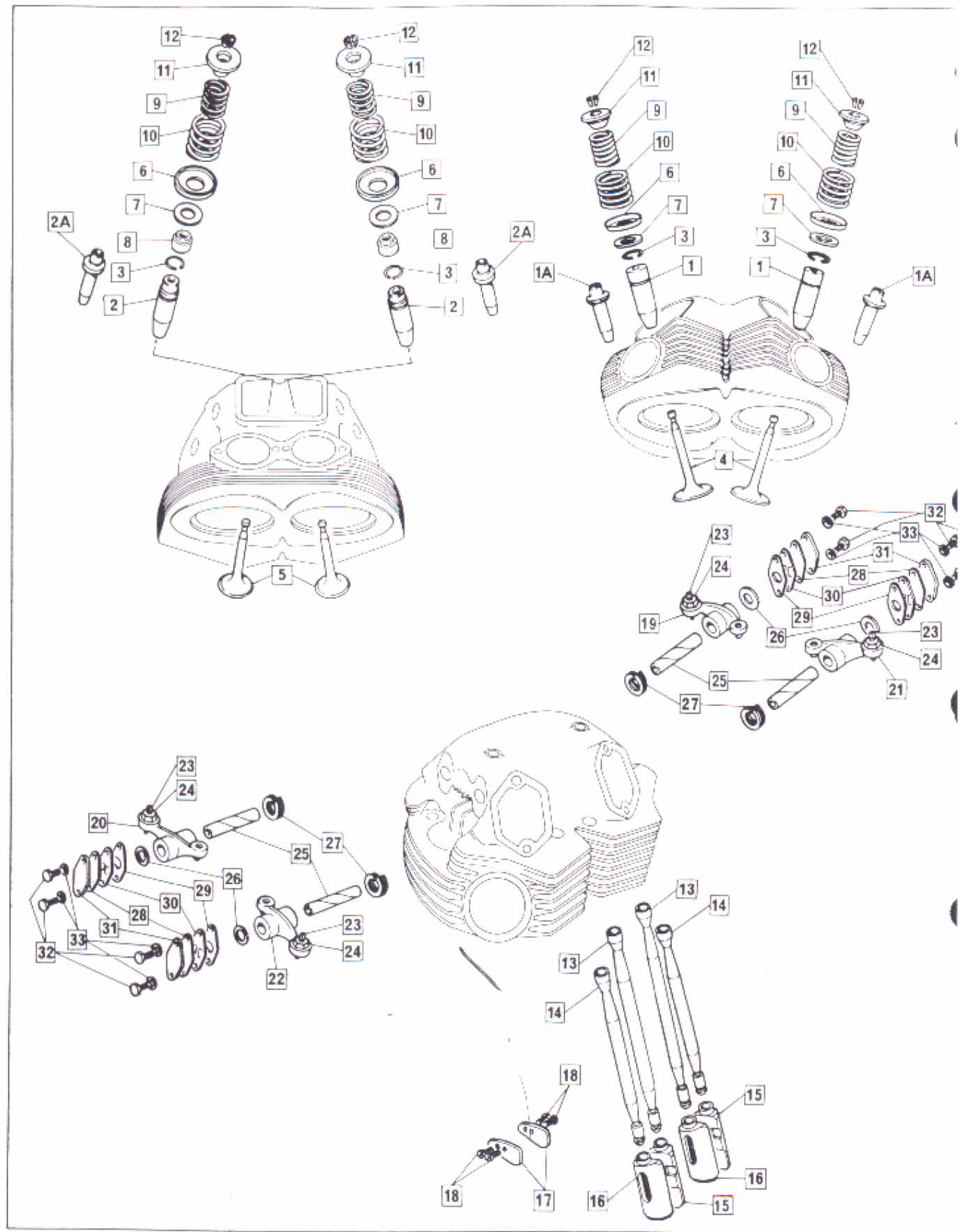
Valve Gear
