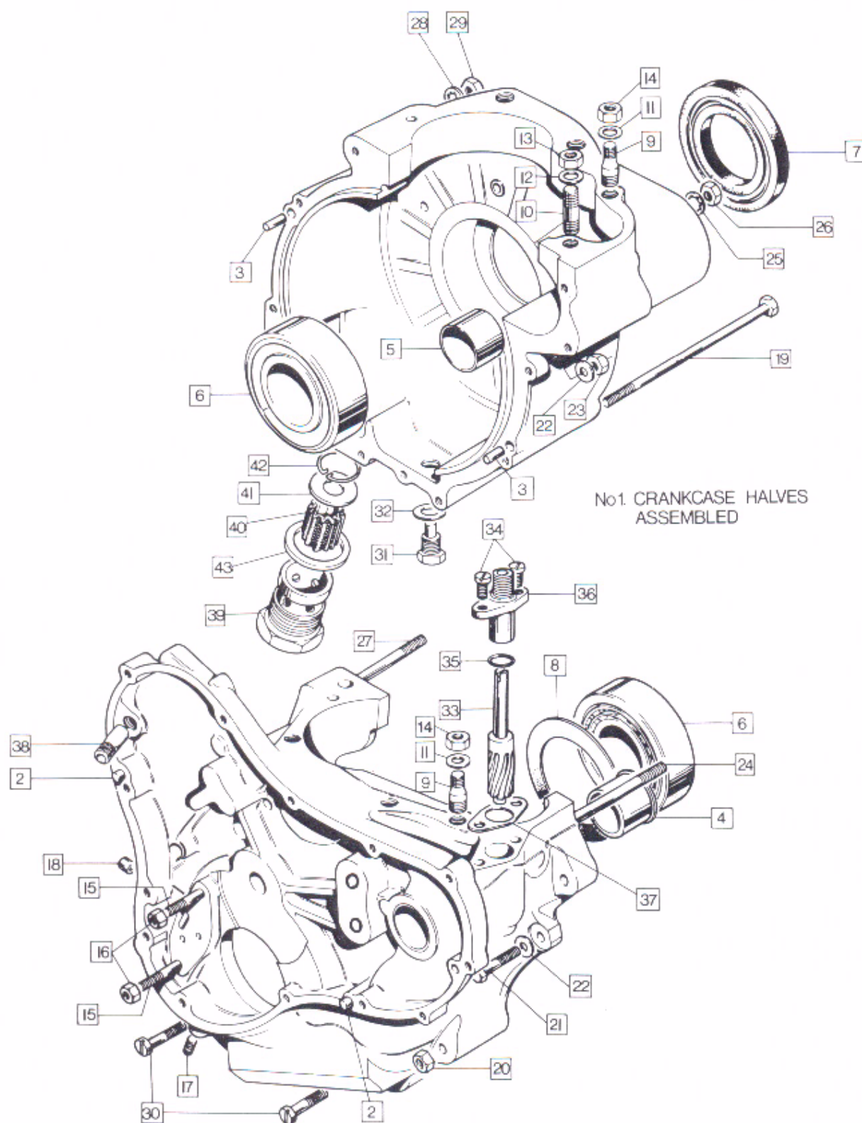
850 Engine: Crankcases, Filter, Breather, Tachometer Drive
