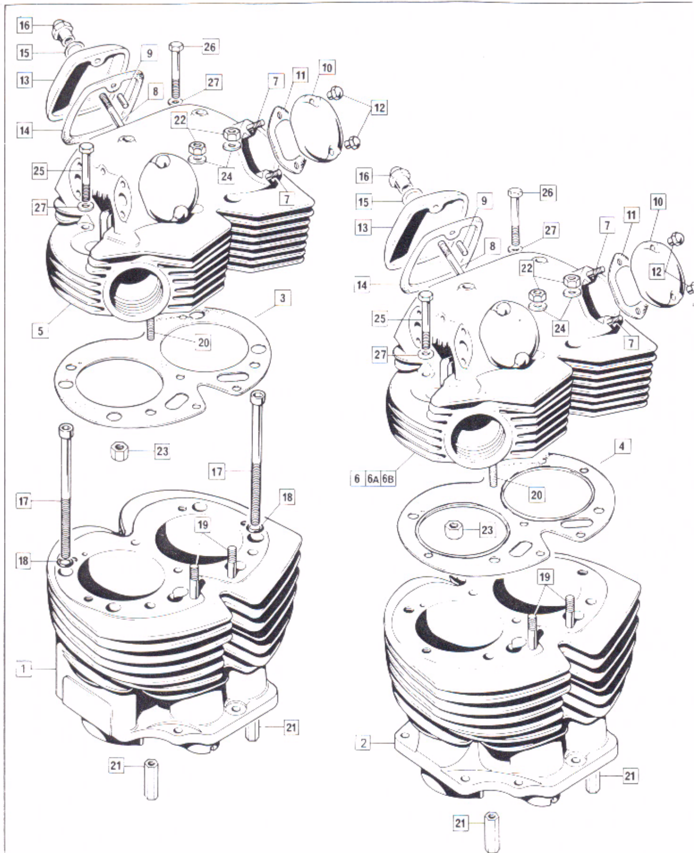
Engine: Cylinder, Cylinder Head 750 and 850
