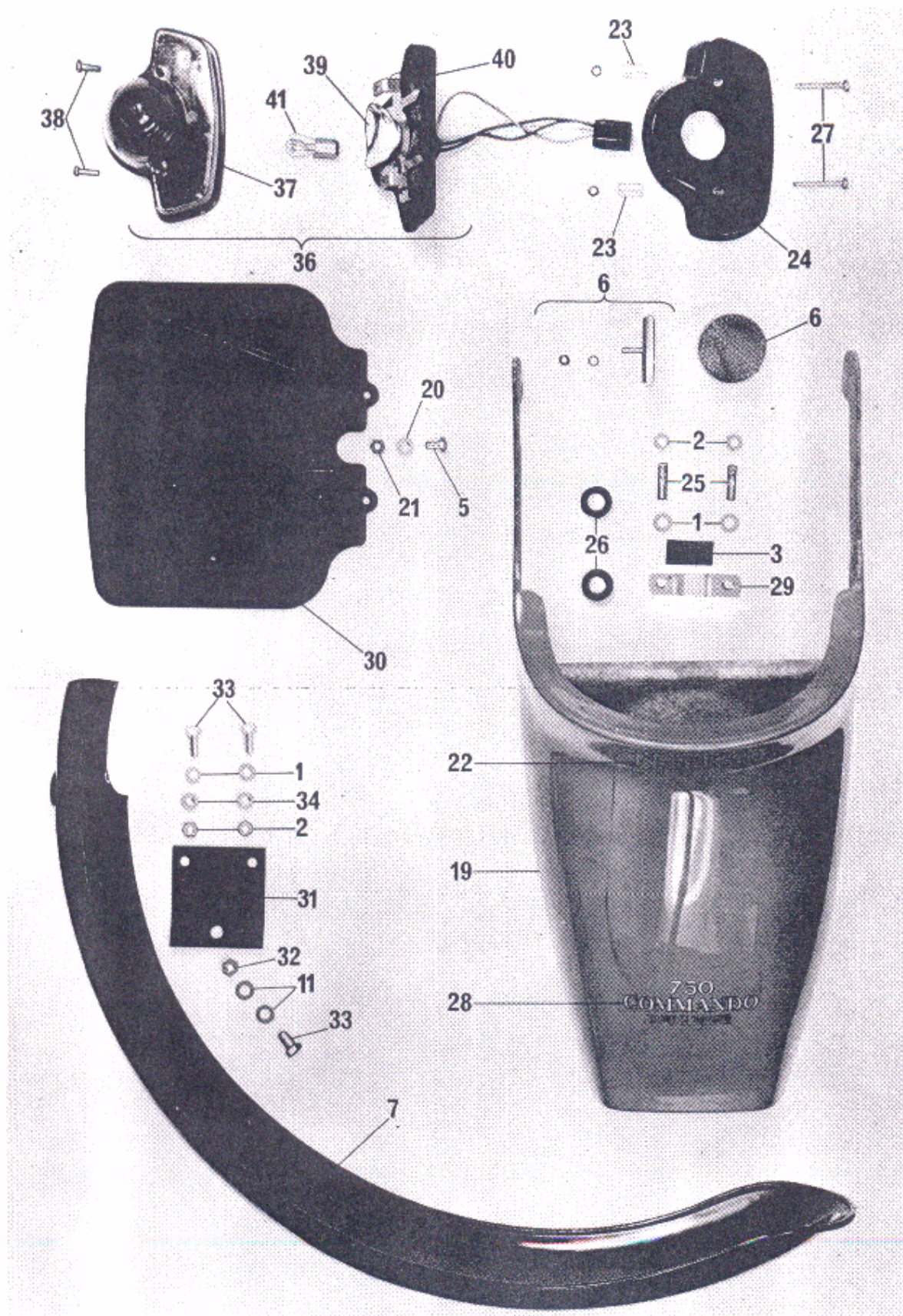
Rear Fenders, Tail Light and Tail Section
