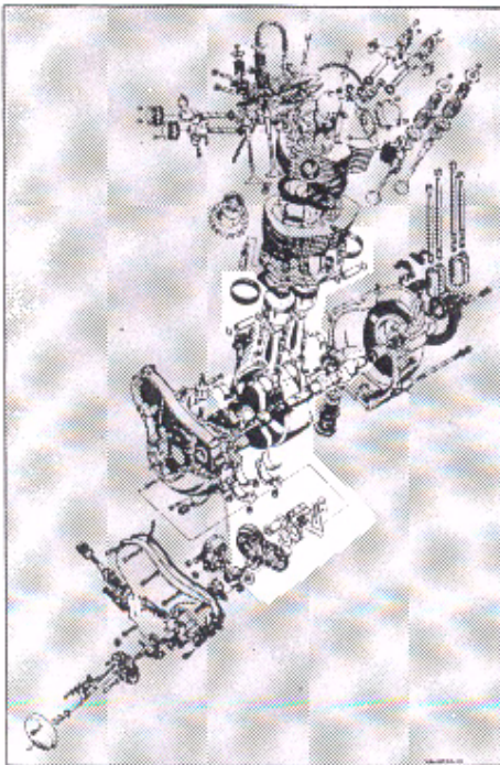
Engine: Crankshaft, Connecting Rods, Pistons, Camshaft, Timing Gear
