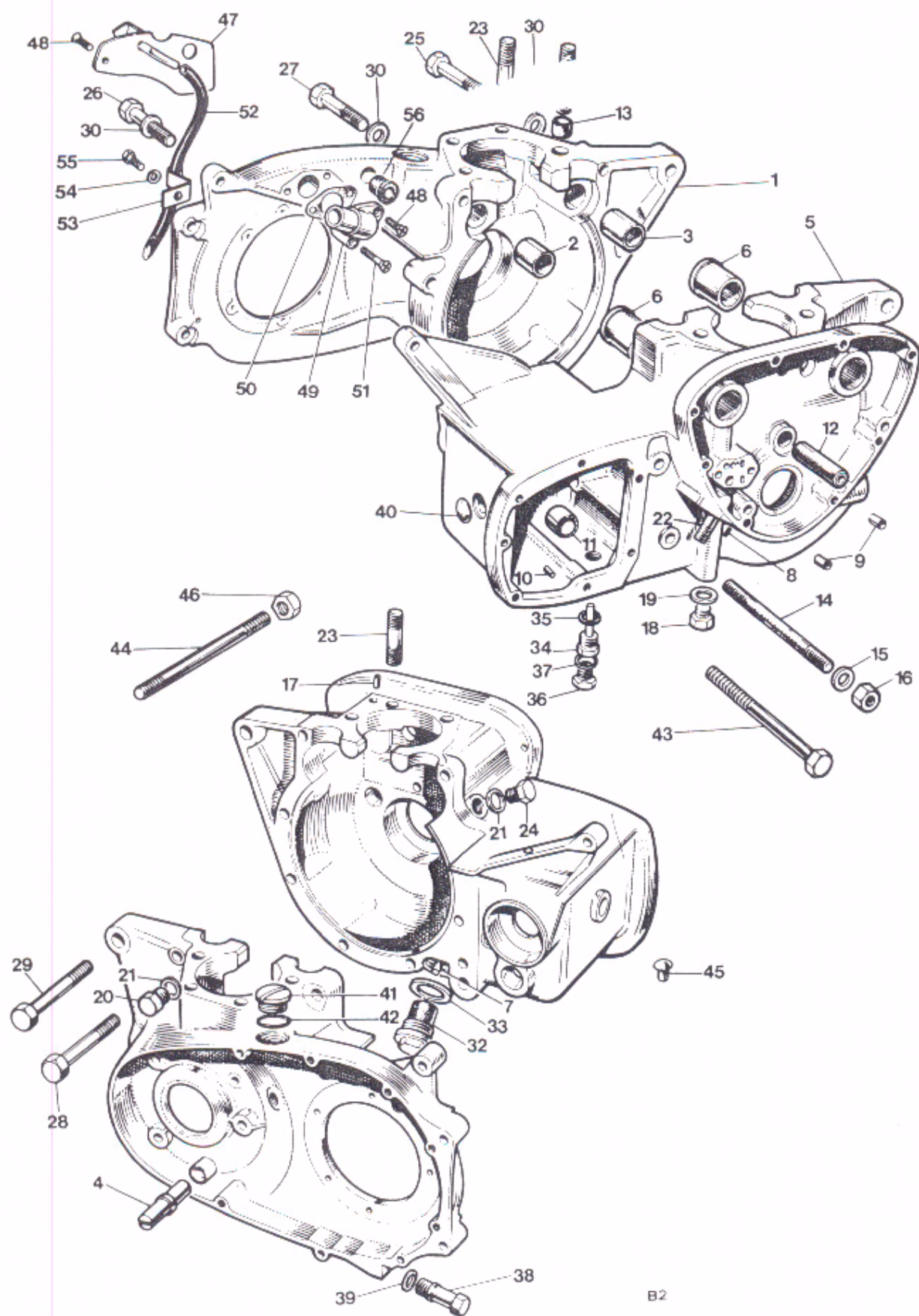
Fig. 2 CRANKCASE
