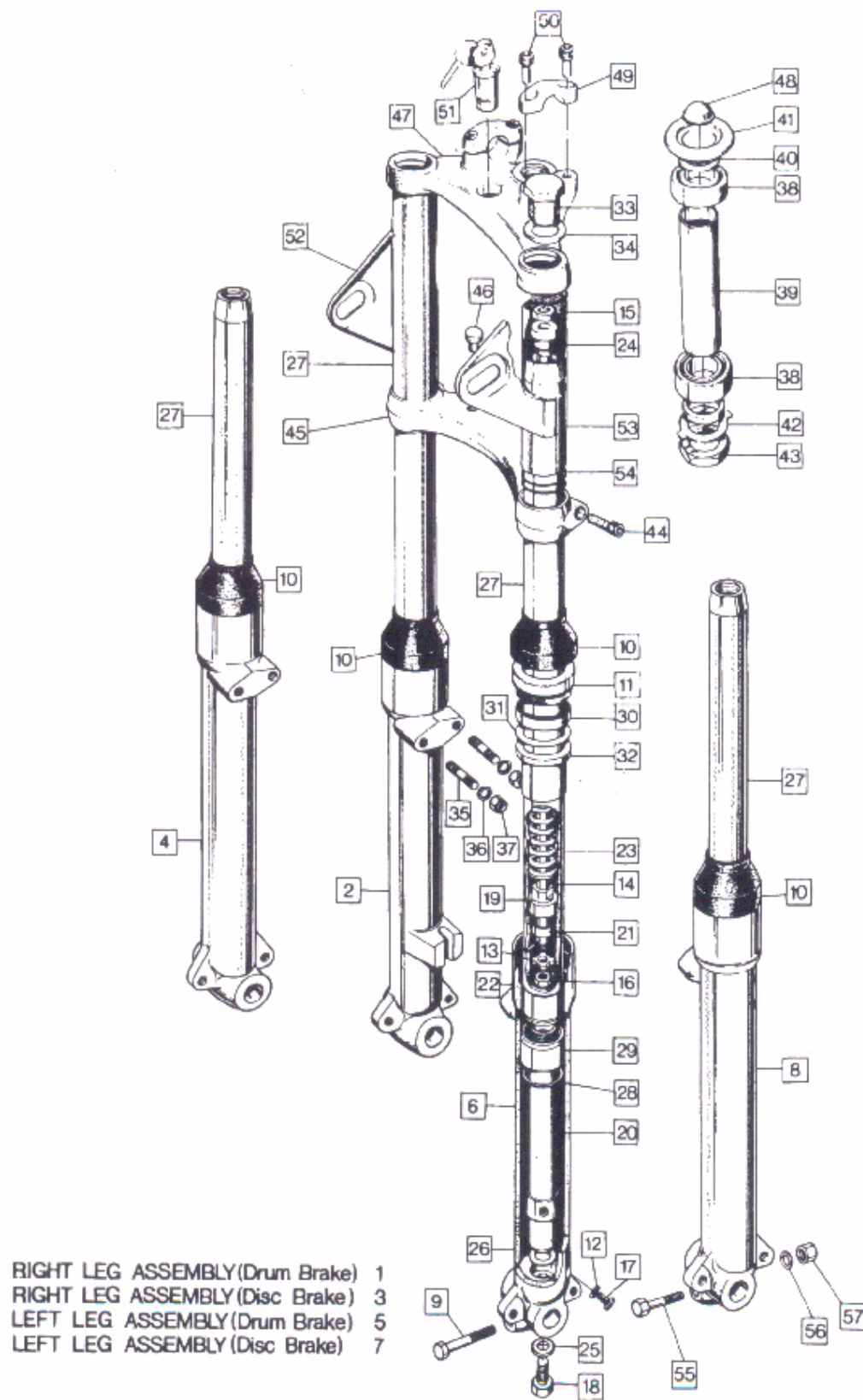
Front Forks, Steering Lock, Steering Head Bearings
