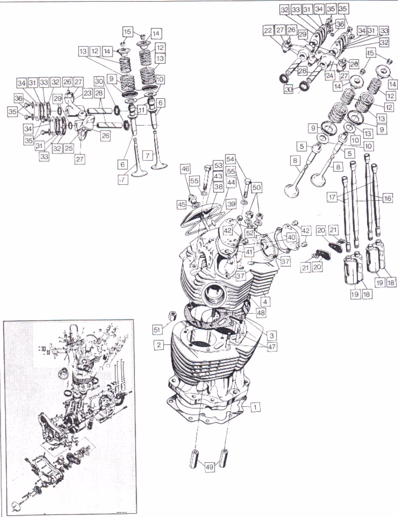
Engine: Cylinder, Cylinder Head and Fittings
