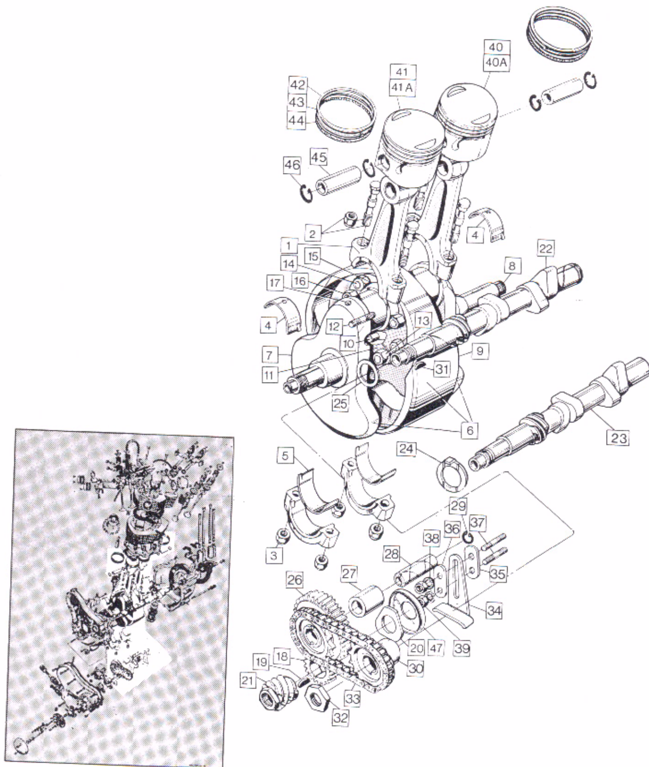
Engine: Crankshaft, Connecting Rods, Pistons, Camshaft, Timing Gear
